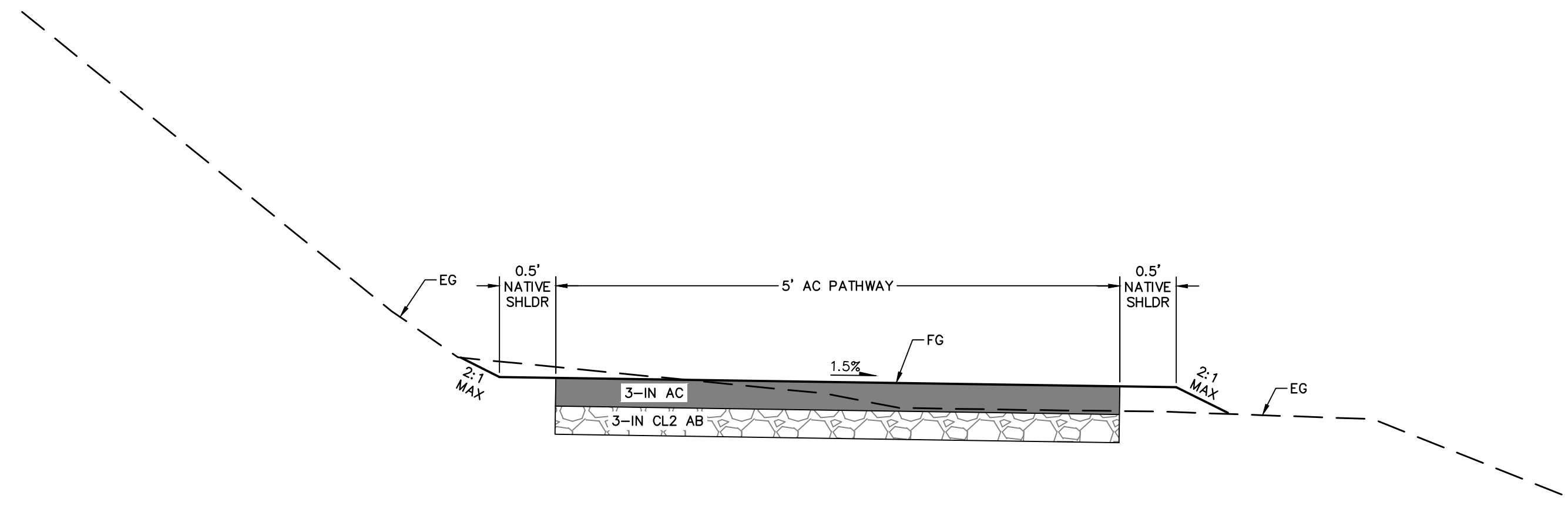
4 - TYPICAL PATHWAY SECTION 4 NTS PATHWAY STA 31+00 - END
