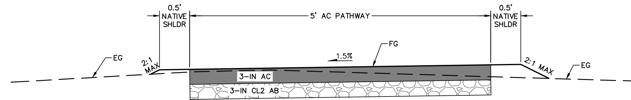
2 - TYPICAL PATHWAY SECTION 2 NTS PATHWAY STA 10+25 - 25+50
