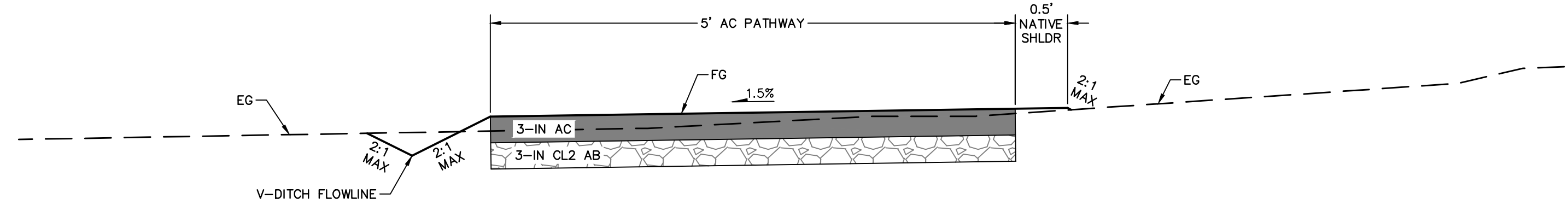
3 - TYPICAL PATHWAY SECTION 3 NTS PATHWAY STA 25+50 - 31+00
