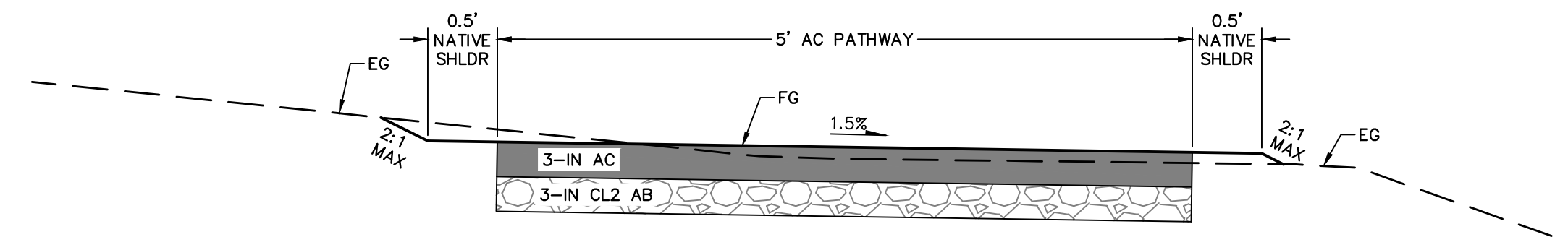
1 - TYPICAL PATHWAY SECTION 1 NTS PATHWAY BEG - STA 10+25
